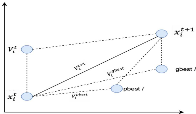
Fig. 3 PSO Searching Concept.
