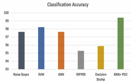
Fig. 5 Classification Accuracy.
