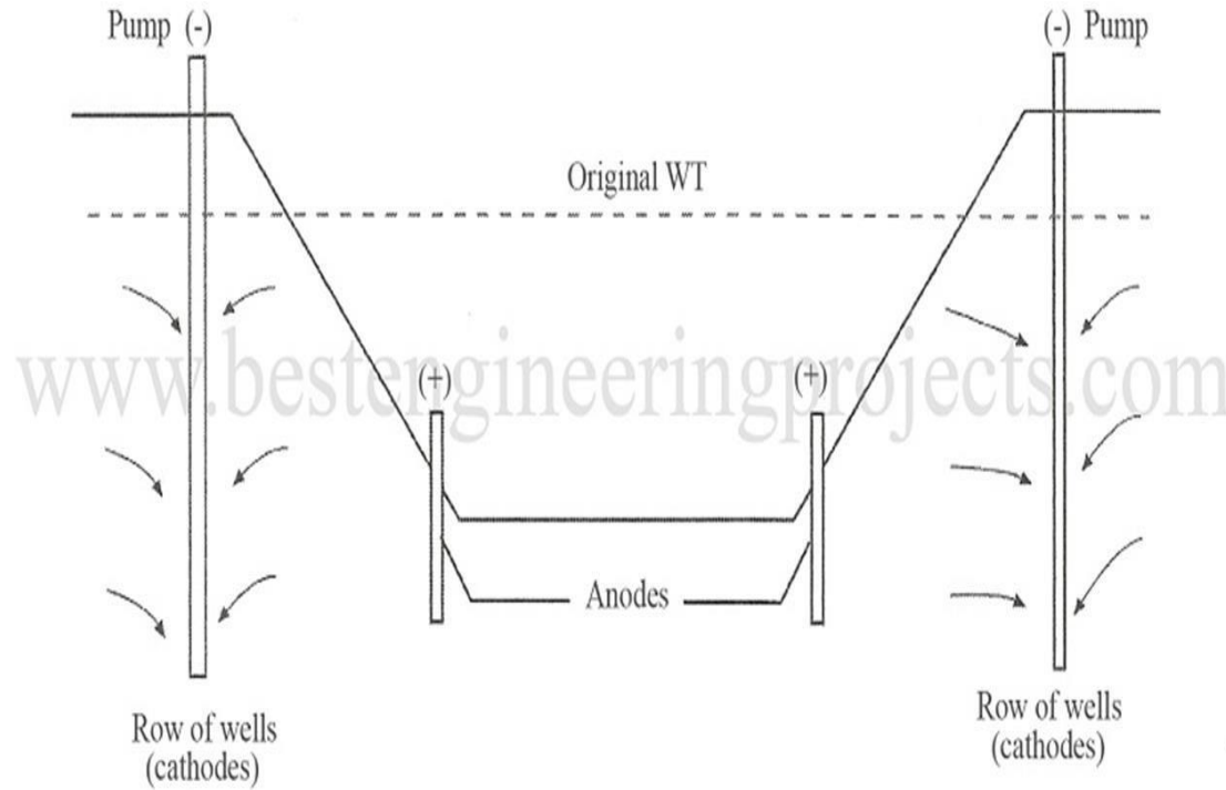
Fig 1 Electro-osmosis Method
