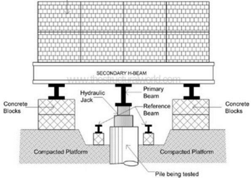
Layers of concrete blocks supported by H-Beam (no. and sizes varies according to required load)
