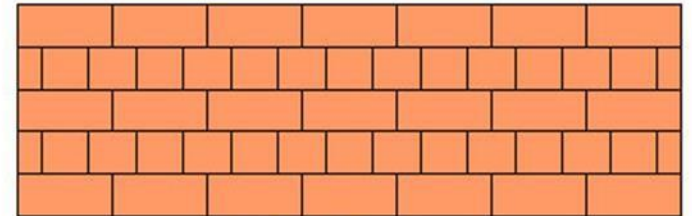
English Bond
